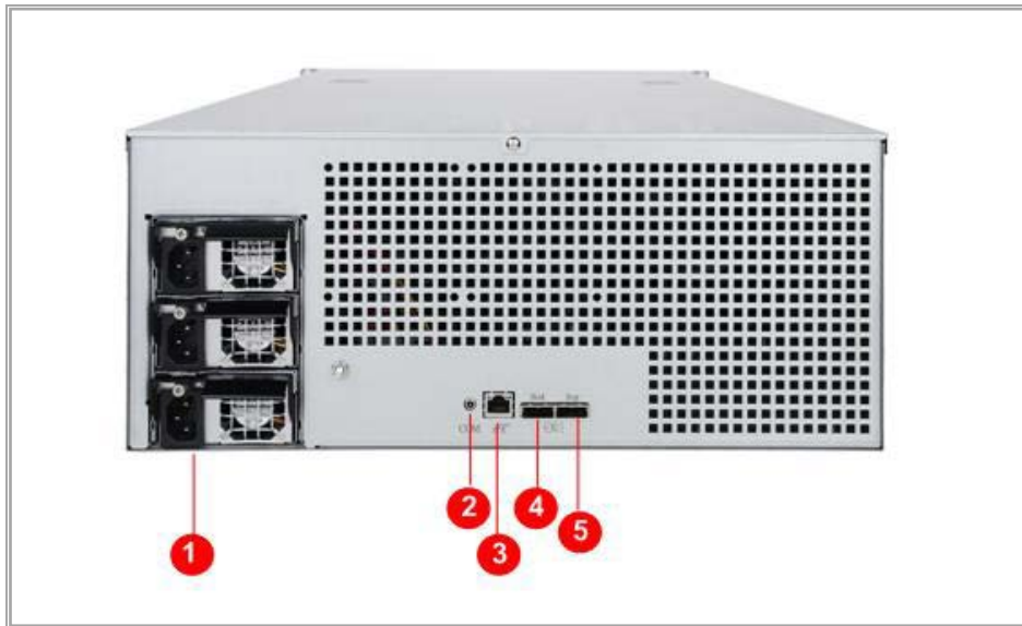
Figure 3-1 24 Slots Device Rear Panel
